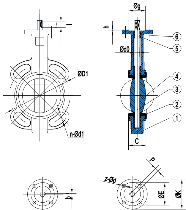
Wafer Butterfly Valve (As2129)
