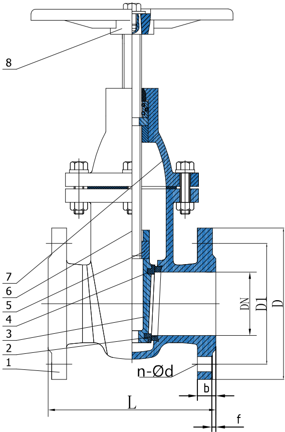
Non-Rising Stem Solid Wedge Gate Valve
