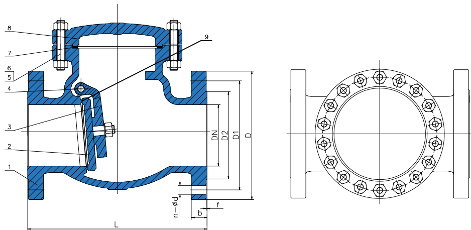
Swing Check Valve
