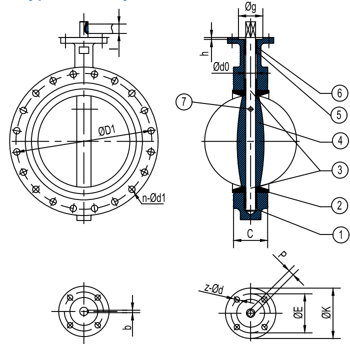
U-Type Butterfly Valve
