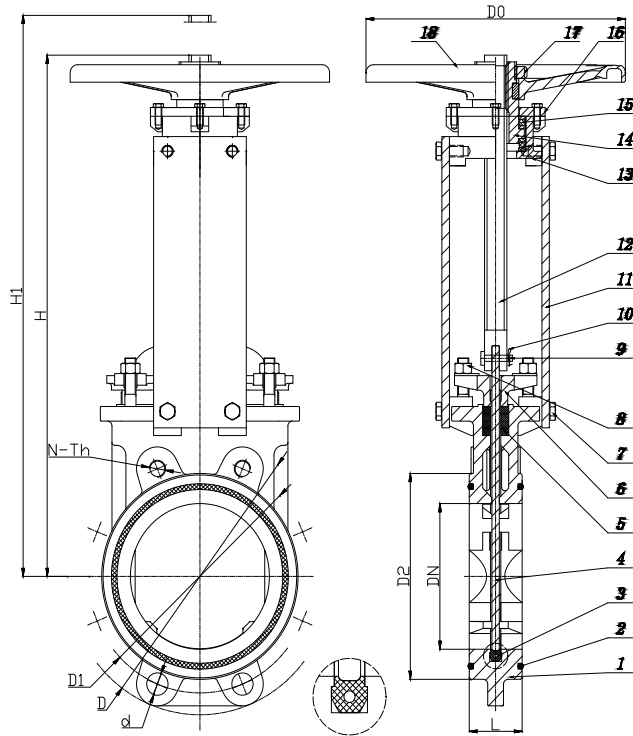
Knife gate valve
